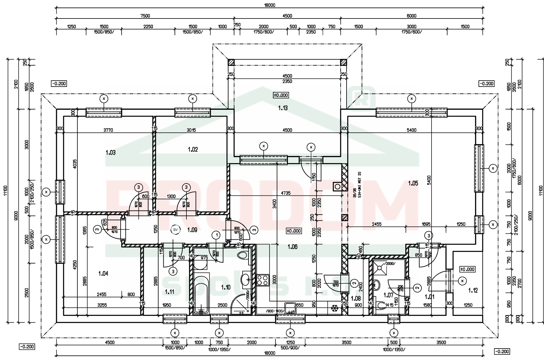
BUNGALOW 182 - Z0
